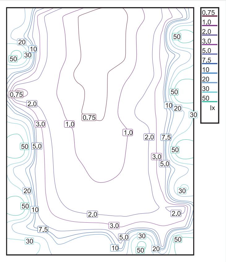
Industrial Area / Calculation surface 4 / Isolines/Horizontal illuminance Calculation surface 4 / Isolines/Horizontal illuminance
