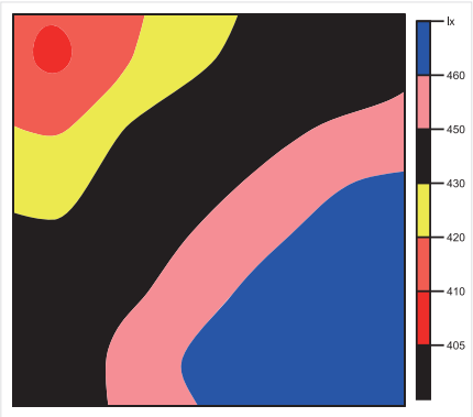
Industrial Area / Office Building / Ground Floor / Calculation surface 3 / False colours/Horizontal illuminance
