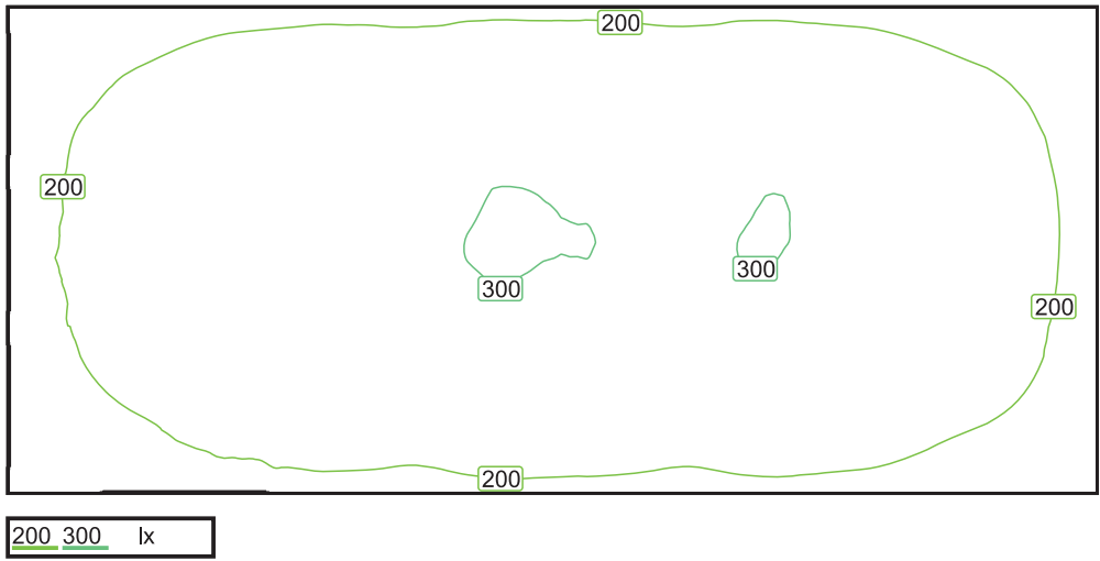
Scale: 1 : 200 Perpendicular illuminance (Surface) Average: 240 lx, Min: 113 lx, Max: 303 lx, Min/average: 0.469, Min/max: 0.371, Points: 1024 x 512 (Relevant: 523586) Height of working plane: 0.800 m, Wall zone: 0.000 m
