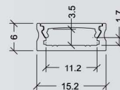
Sectional Dimensions (mm)
